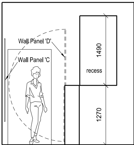
ELEVATION - Recess
